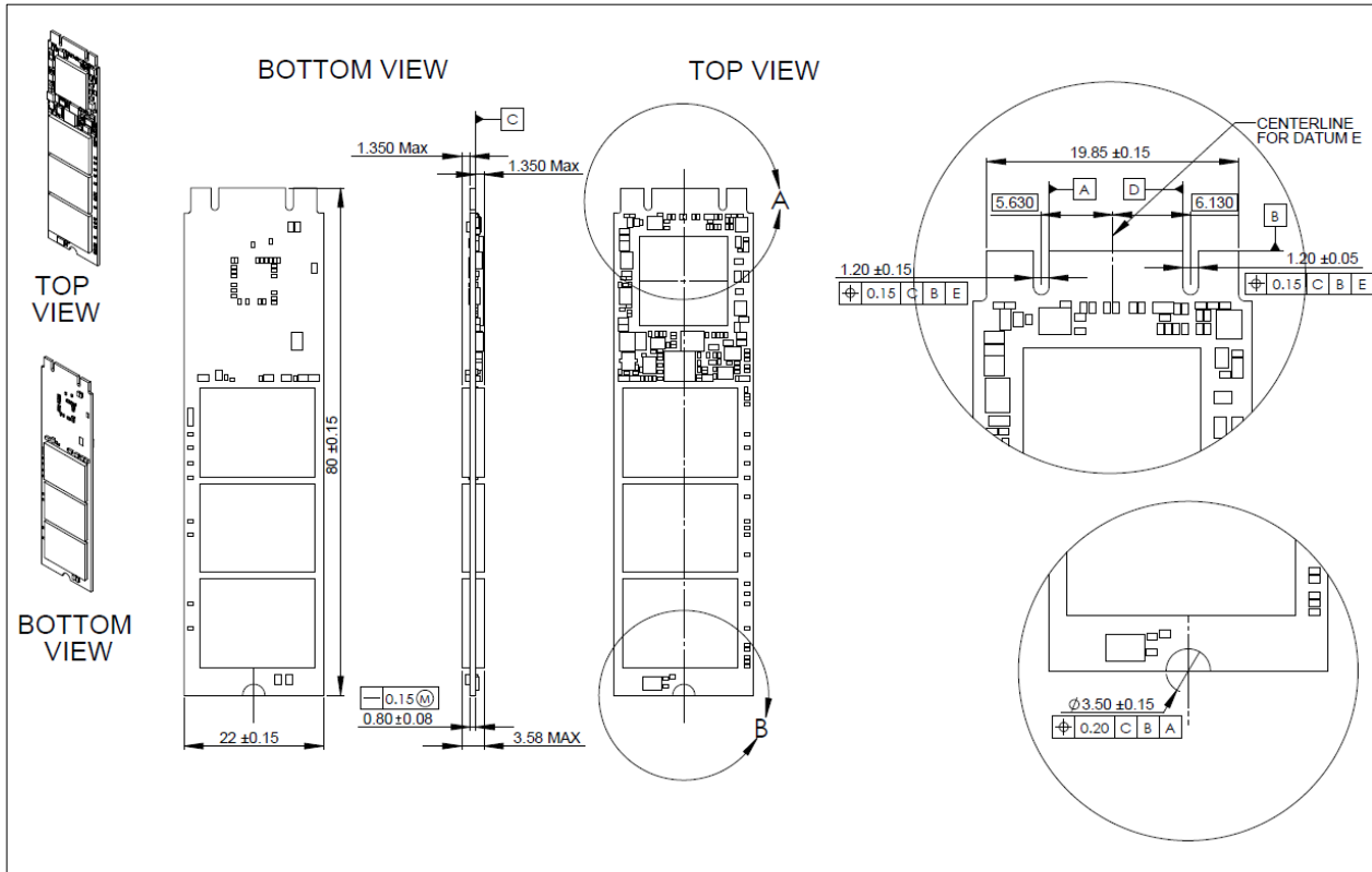
Figure 2: Dimensions for 60 mm double-sided M.2 Form Factor Drives (2260-D2-B-M) 180GB and 240GB
